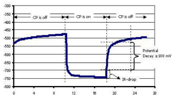
Figure 2. Polarisation curve from CP-system
